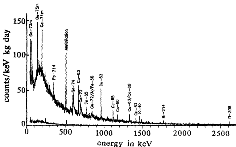
Figure 4 Background spectra of similar Ge spectrometers (0.9 kg active volume) with passive and active shielding at sea level (top) and at 15 m.w.e. (bottom).
